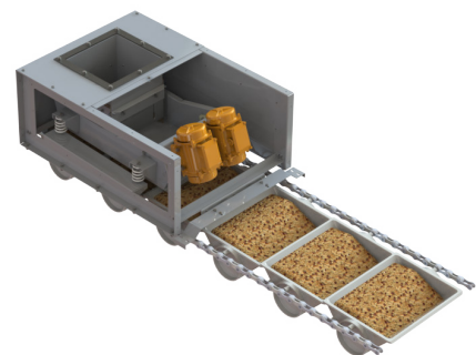
Vibrating feeder Traditional gentle feeding system for most product types. Filling degree up to 65%
