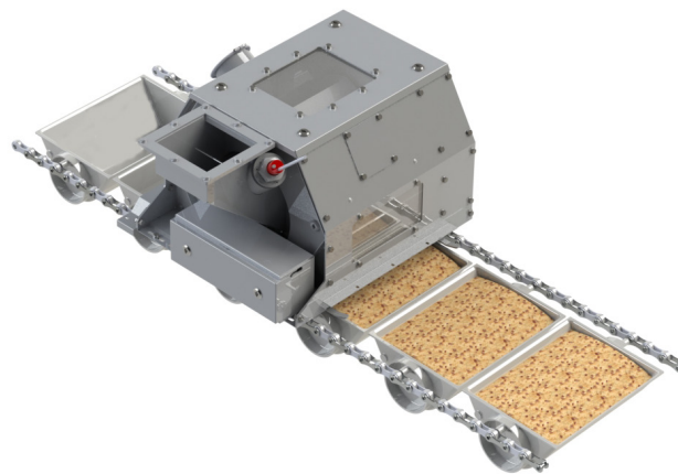
Drum feeder
