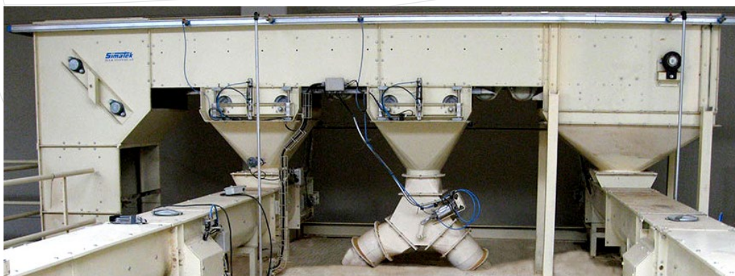
Elevator type 200 with two intermediate outlets
